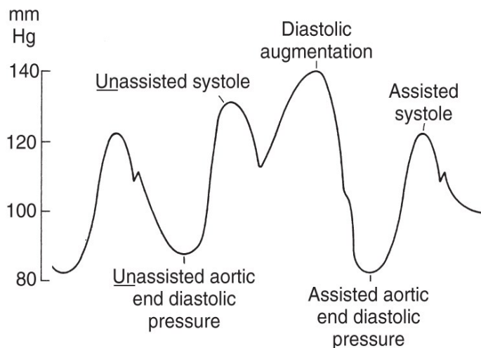
Figure 6.2 Correct IABP Timing. (Courtesy of MAQUET Cardiovascular, LLC, Wayne, NJ.) Used with permission (El Sevier 2019)
